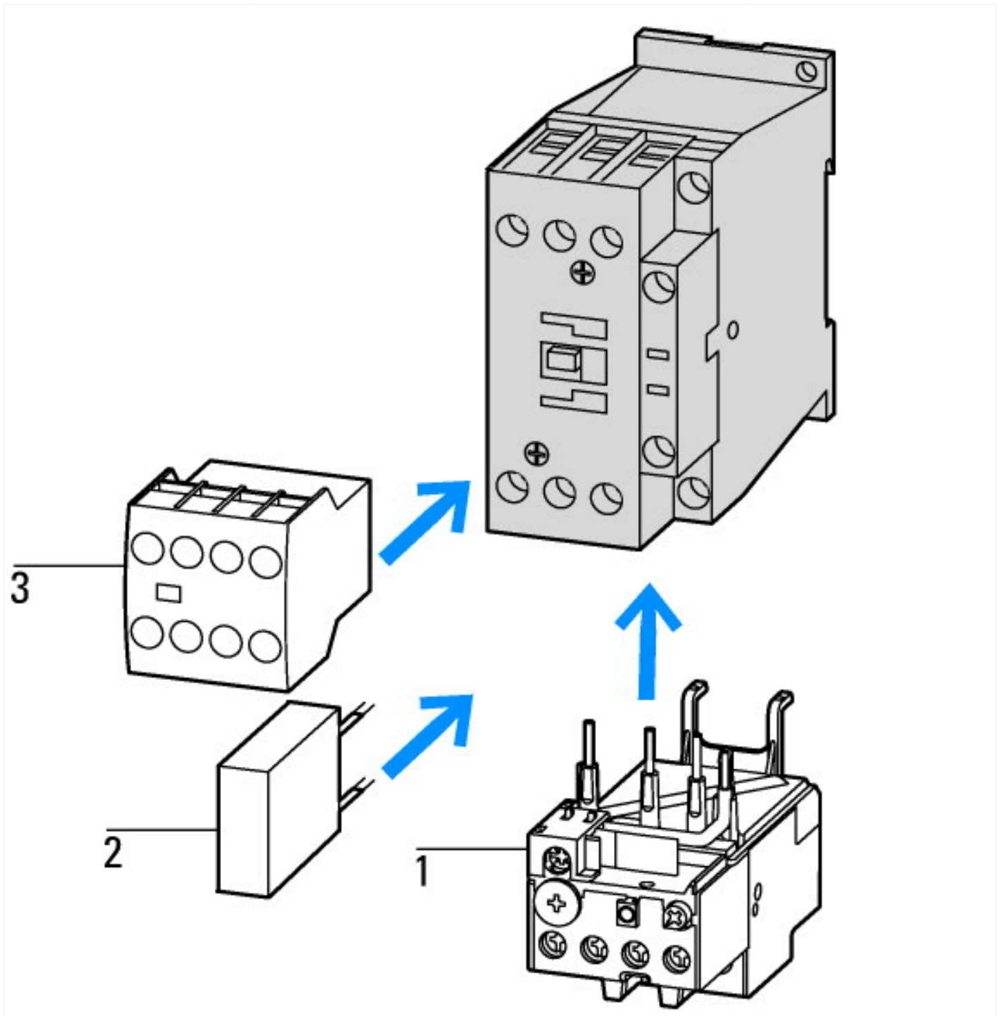
1: Motorschutzrelais
